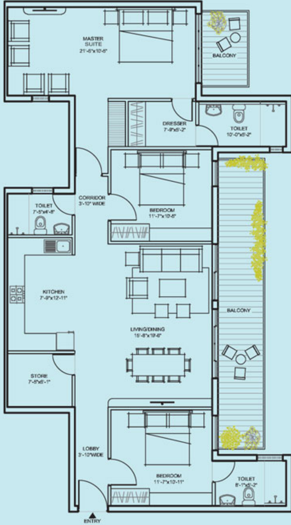
OPTION 1 3BR3T WITH MASTER SUITE LIVING/DINING MASTER SUITE WITH WALK-IN DRESSER OPEN KITCHEN STORE/PUJA ROOM 2 SIT-OUT BALCONIES
